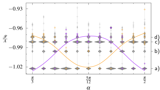
Fig. 6 The distribution of the free energy per area \mathcal{F}/A is shown as a function of angle \alpha for parameters that stabilize quasicrystals. The cross symbols show the outcomes of independent simulation runs and the surrounding shapes are violin plots, in which the width gives the frequency of the respective value. The full distribution contains different values of the tilt \gamma between the initial grain boundaries and the box. The solid lines are guides that highlight the trends in the colored data. These are the distributions restricted to the extreme cases of tilt angles \gamma = 0 (orange) and \gamma = \frac{\pi}{12} (purple). Exemplary configurations for the free energies labeled (a) through (d) on the right are shown in Fig. 7.
