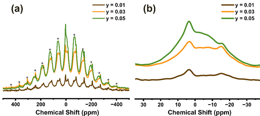
Fig. 3 (a) {}^7\text{Li} NMR spectra of \text{Zn}_{0.91-y}\text{Eu}_{0.09}\text{Li}_{0.03}\text{MoO}_4 ( y = 0.01, 0.03, \text{ and } 0.05 ). (b) Magnified view of the isotropic peak for detailed observation.
