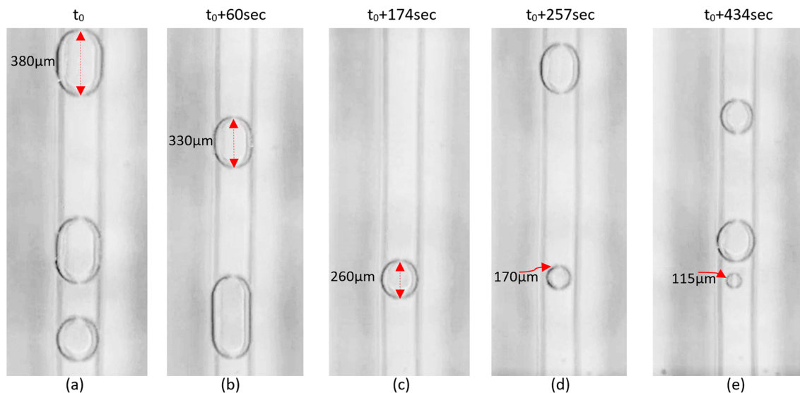
Fig. 7 Dynamics of a bubble (same bubble from a to e) moving within the microchip highlighting \text{CO}_2 gas dissolution in water: (a) movement of \text{CO}_2 bubble (size 380\ \mu\text{m} ; red arrow); (b) movement of \text{CO}_2 bubble (size reduction to 330\ \mu\text{m} ); (c–e) gas bubble size reduction versus time ( 260 , 170 , and 115\ \mu\text{m} , respectively).
