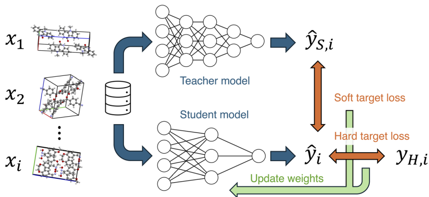
Fig. 1 Knowledge distillation of neural networks. Teacher and student models are the two neural network potentials, PFP and CHGNet, respectively, in this work. Hard target is the energy and force of organic crystals in the MPtrj dataset, and the soft target is those calculated by the PFP model for the same structures. The prediction value of the student model is used to calculate the total loss for hard and soft targets to update weights of the student model.
