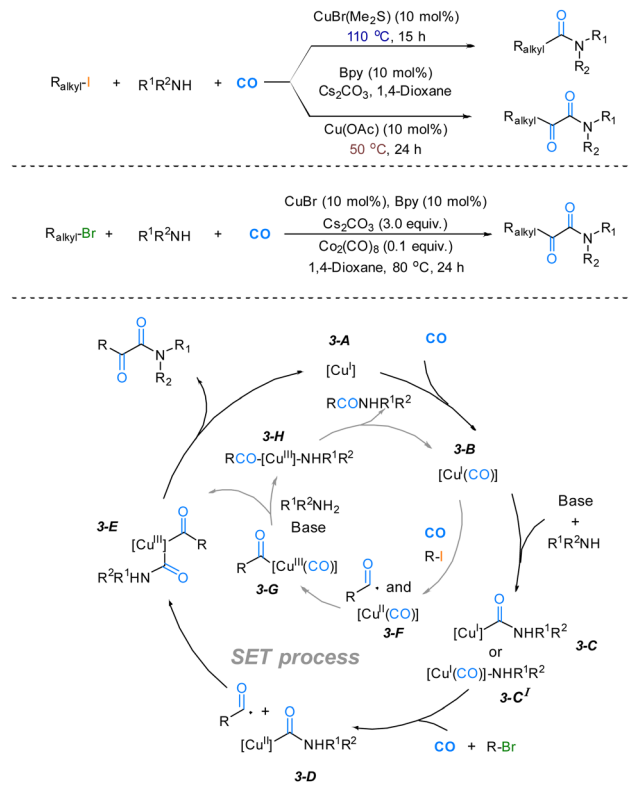
Fig. 3 Copper-catalyzed direct mono- and double-carbonylation reactions.
