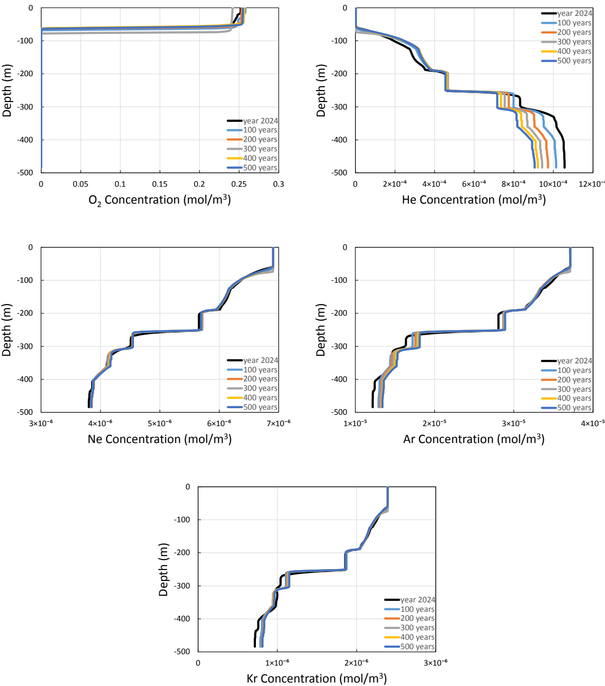
Fig. 10: Predicted future vertical profiles of O 2 , He, Ne, Ar, and Kr concentrations in the lake.
