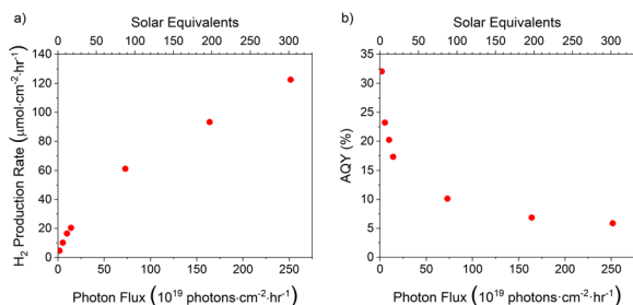
Fig. 1 (a) Hydrogen production rate and (b) AQY of the photocatalyst sheet at an ambient temperature of 23 °C under increasing photon flux.
