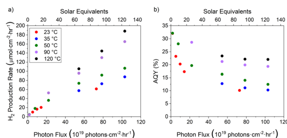
Fig. 2 (a) Hydrogen production rate and (b) AQY of the photocatalyst sheet in the temperature range 23–120 °C.
