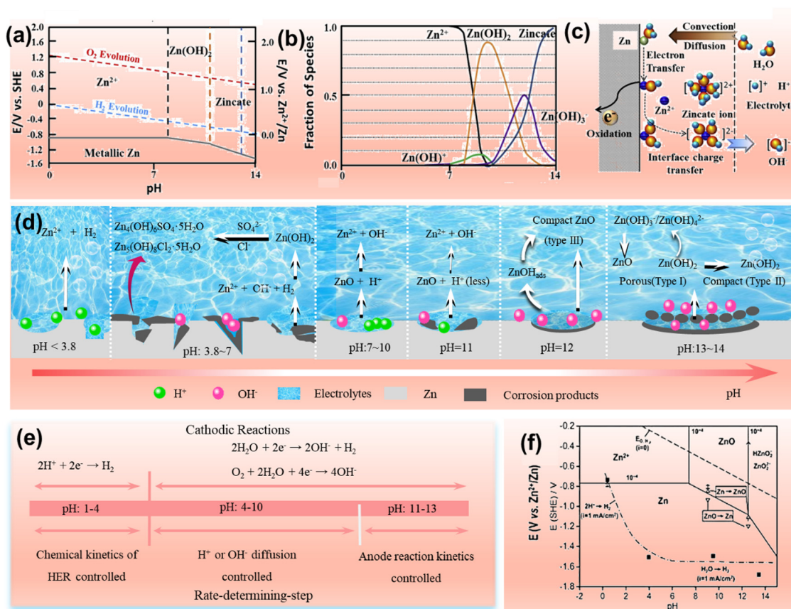
Fig. 2 (a) Pourbaix diagram of Zn– \text{H}_2\text{O} at 25 °C. (b) Fraction Zn species at different pH values. (c) Dissolution process illustration of Zn. Reproduced from ref. 38 with permission from Elsevier, copyright 2020. (d) Various Zn corrosion modes at different pH values. (e) Illustrations of cathodic reactions and rate-determining steps of Zn corrosion. (f) Pourbaix diagram with the consideration of kinetics factors for 10^{-4} mol \text{L}^{-1} \text{Zn}^{2+} . Reproduced from ref. 39 with permission from Elsevier, copyright 1991.
