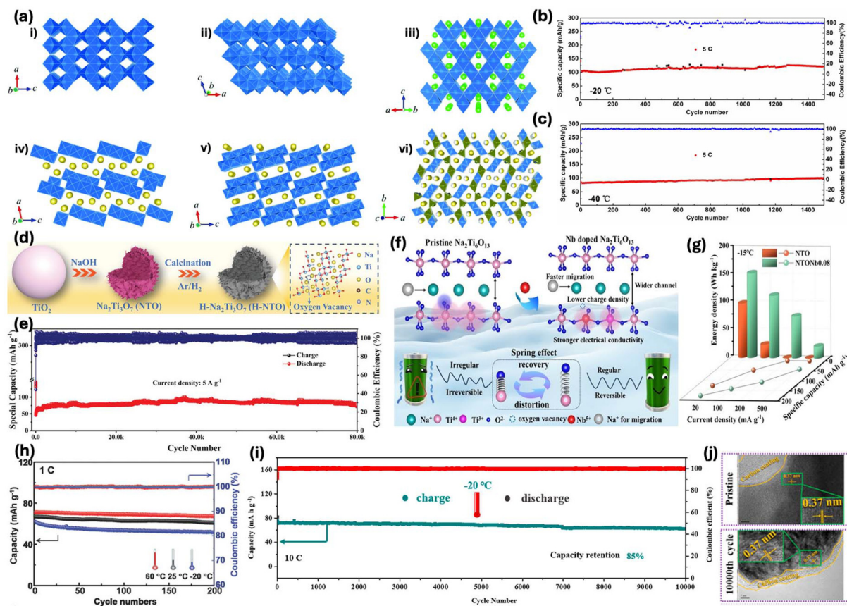
Fig. 13 (a) Schematic crystal structures of typical Ti-based compounds for sodium storage: (i) anatase \text{TiO}_2 , (ii) \text{TiO}_2 -B, (iii) spinel \text{Li}_4\text{Ti}_5\text{O}_{12} , (iv) \text{Na}_2\text{Ti}_3\text{O}_7 (zig-zag), (v) \text{Na}_2\text{Ti}_6\text{O}_{13} (zig-zag), and (vi) tunnel-type \text{Na}_4\text{Mn}_4\text{Ti}_5\text{O}_{18} . \text{TiO}_6 octahedra and \text{MnO}_5/\text{MnO}_6 polyhedra are shown in blue and olive, with Li and Na as green and yellow spheres. 199 Charge-discharge capacities of \text{TiO}_2 @rGO at 5C for (b) -20^\circ\text{C} , and (c) -40^\circ\text{C} over cycling. 201 (d) Schematic of the synthesis route and (e) long-term cycling performance of H-NTO microspheres at 5\text{ A g}^{-1} . 202 (f) Schematic illustration of crystal structure evolution in NTO before and after Nb doping. (g) Rate performance and energy density comparison of NTO and \text{NTO}_{0.08}\text{Nb} at 100\text{ mA g}^{-1} under -15^\circ\text{C} . 48 (h) Cycling stability of \text{NaV}_{1.25}\text{Ti}_{0.75}\text{O}_4/\text{Na}_{0.8}\text{Ni}_{0.4}\text{Ti}_{0.6}\text{O}_2 full cells at 1C. 204 (i) Extended cycling of \text{NaTi}_2(\text{PO}_4)_3/\text{Ni}(\text{OH})_2 at -20^\circ\text{C} and 10C rate; (j) TEM images of NTP@C electrode at initial and 10 000th cycle. 209
