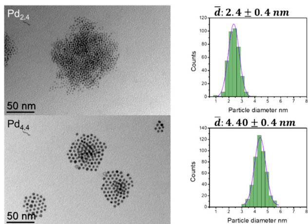
Fig. 2 TEM images of the monodispersed 2.4 \pm 0.4 nm and 4.4 \pm 0.4 nm Pd p-NP .
