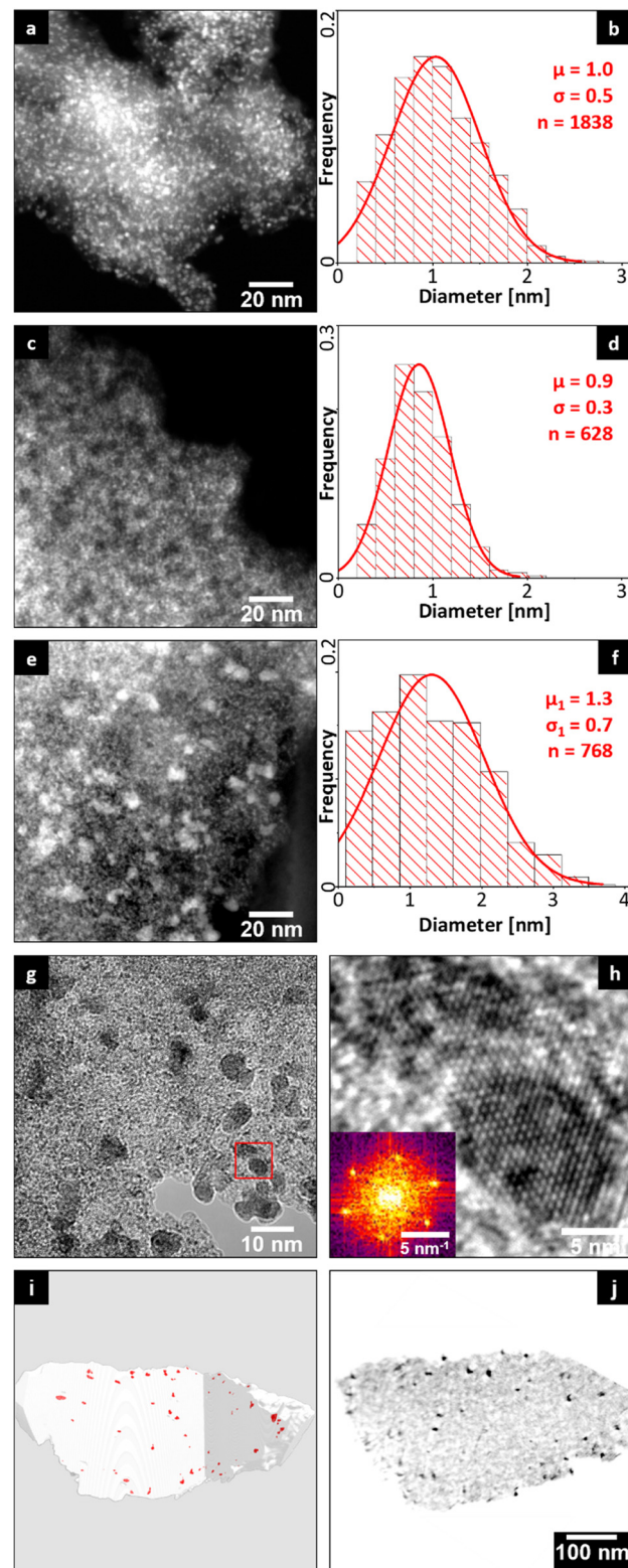
Fig. 3 HAADF-STEM images with bright Ru nanoparticles and corresponding PSDs of a) commercial 5 wt% Ru/AC catalyst (PSD in b), c) Ru PTA /CTF3 (PSD in d), and e) Ru PTA /CTF3 after 6th recycling run, f) bimodal PSD of individual (background plot) and coalesced (inset) Ru particles from e), g) and h) HRTEM of coarsened Ru particles with dark crystallographic contrast, i) STEM tomography reconstruction: iso-surfaces of coarsened Ru particles (red) embedded within the open-porous CTF support (transparent grey), j) orthoslice (cross-section) of reconstruction with dark Ru agglomerates.
