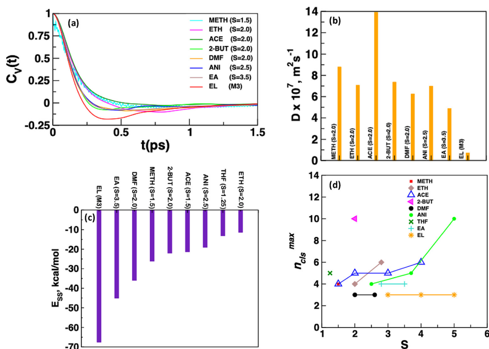
Fig. 2 (a) Velocity autocorrelation function plot of carbamazepine (CBZ) molecules, (b) diffusion coefficient of CBZ molecules at the lowest supersaturation in different solvents, (c) E_{SS} (kcal mol ^{-1} ) solvent–solvent interaction energy per solvent molecule in low supersaturation systems in different solvents and (d) largest size ( n_{\text{cls}}^{\text{max}} ) of the CBZ cluster as a function of supersaturation in different solvents.
