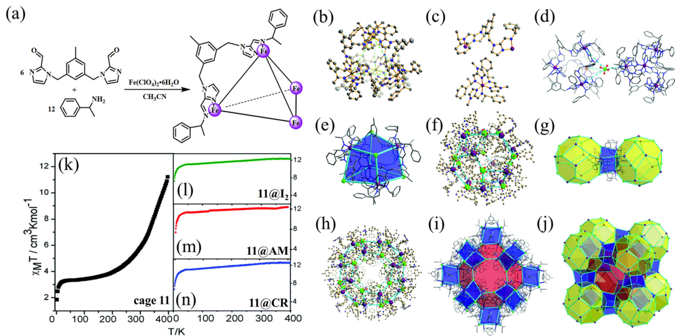
Fig. 11 Synthesis method (a) and crystal structure of cage 11 . (c) One edge and one vertex of cage 11 . (d) Two adjacent cages bridged through a \text{ClO}_4^- anion. (e) Diagram of double 4-rings. (f) Diagram of \beta -cage. (g) Diagram of two \beta -cage attached to a double 4-rings. (h) Diagram of \alpha -cage. (i) Diagram of 12 double-4 rings around each \alpha -cage. (j) Diagram of LTA topology. \chi_m T vs. T plots for 11 (k), 11@I 2 (l), 11@AM (m) and 11@CR (n). 82
