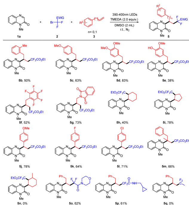
Scheme 3 Substrate scope of alkenes and difluoroalkyl bromides. Reaction conditions: 1a (0.2 mmol), 2 (0.4 mmol), 3 (0.4 mmol), TMEDA (0.4 mmol), DMSO (2.0 mL), room temperature, \text{N}_2 , and 24 h. Isolated yield.
