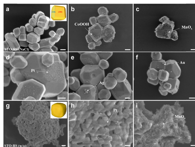
Fig. 2 SEM images of (a) STO:RS(NaCl) and (b) STO:RS(NaCl) loaded with (b) \text{CoOOH} , (c) \text{MnO}_x , (d) Pt, (e) Ag, and (f) Au by photodeposition. SEM images of (g) STO:RS(w/o) and (h) STO:RS(w/o) loaded with (h) Pt and (i) \text{MnO}_x by photodeposition; the scale is 100 nm.
