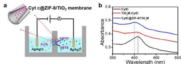
Fig. 11 (a) Schematic illustration of \text{Cyt c}@ZIF-8/\text{TiO}_2 membrane in electrocatalysis cell and its working mechanism. (b) UV-Vis diffuse reflectance spectra of Cyt c (black), \text{TiO}_2 membrane-Cyt c (red), and \text{Cyt c}@ZIF-8/\text{TiO}_2 membrane (blue) with high-purity \text{BaSO}_4 employed as the background. Reproduced with permission from ref. 60.
