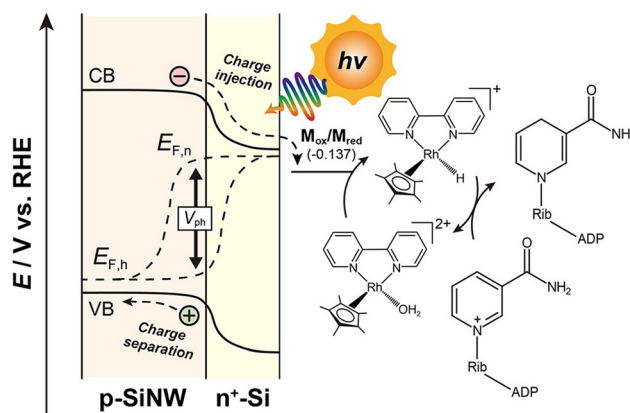
Scheme 9 Reaction scheme of photocatalytic production of NADH at the photocathode driven by n^+p -SiNWs. Reprinted with permission from ref. 69. Copyright 2023, American Chemical Society.
