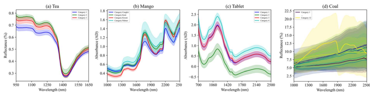
Fig. 4 Presents the raw spectra of (a) tea, (b) mangoes, (c) tablets, and (d) coal, respectively, illustrating the mean \pm standard deviation of samples from various varieties. The curves depicted are averages of the spectra, with the upper and lower boundaries of the translucent areas indicating the \pm standard deviation.
