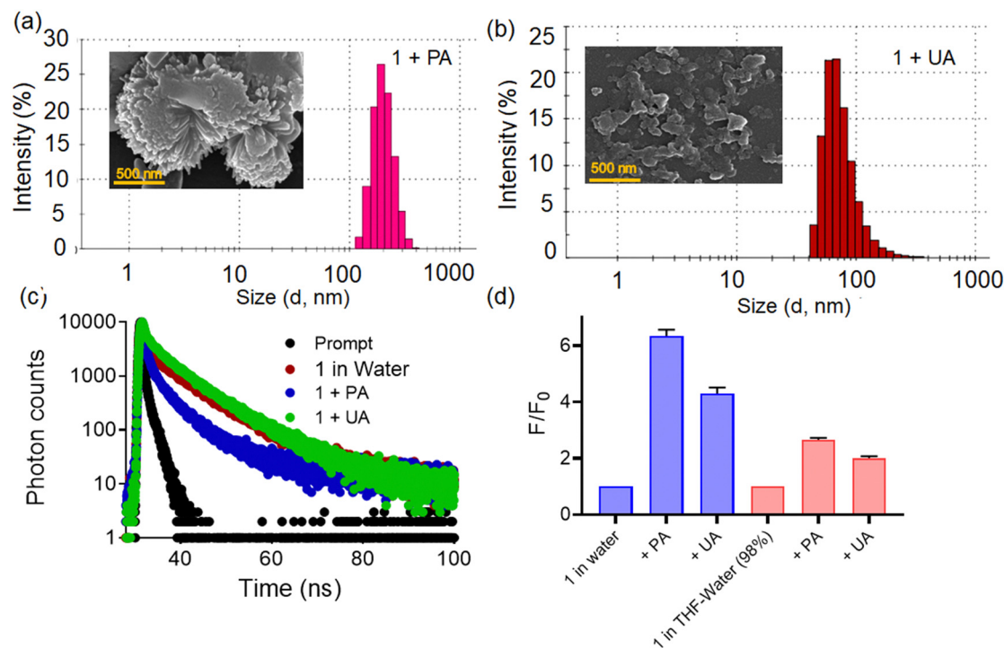
Fig. 6 (a) DLS and FESEM images of 1 with phytic acid in an aqueous medium. (b) DLS and FESEM images of 1 with uric acid in an aqueous medium. (c) Fluorescence lifetime of 1 (10 \mu\text{M} , \lambda_{\text{ex}} = 340 nm) in the presence of phytic acid (60 \mu\text{M} ) and uric acid (100 \mu\text{M} ) in an aqueous medium at 480 nm and 415 nm respectively. (d) Change in fluorescence intensity of 1 in THF-water (98%) and water medium upon addition of phytic acid (60 \mu\text{M} ) and uric acid (100 \mu\text{M} ).
