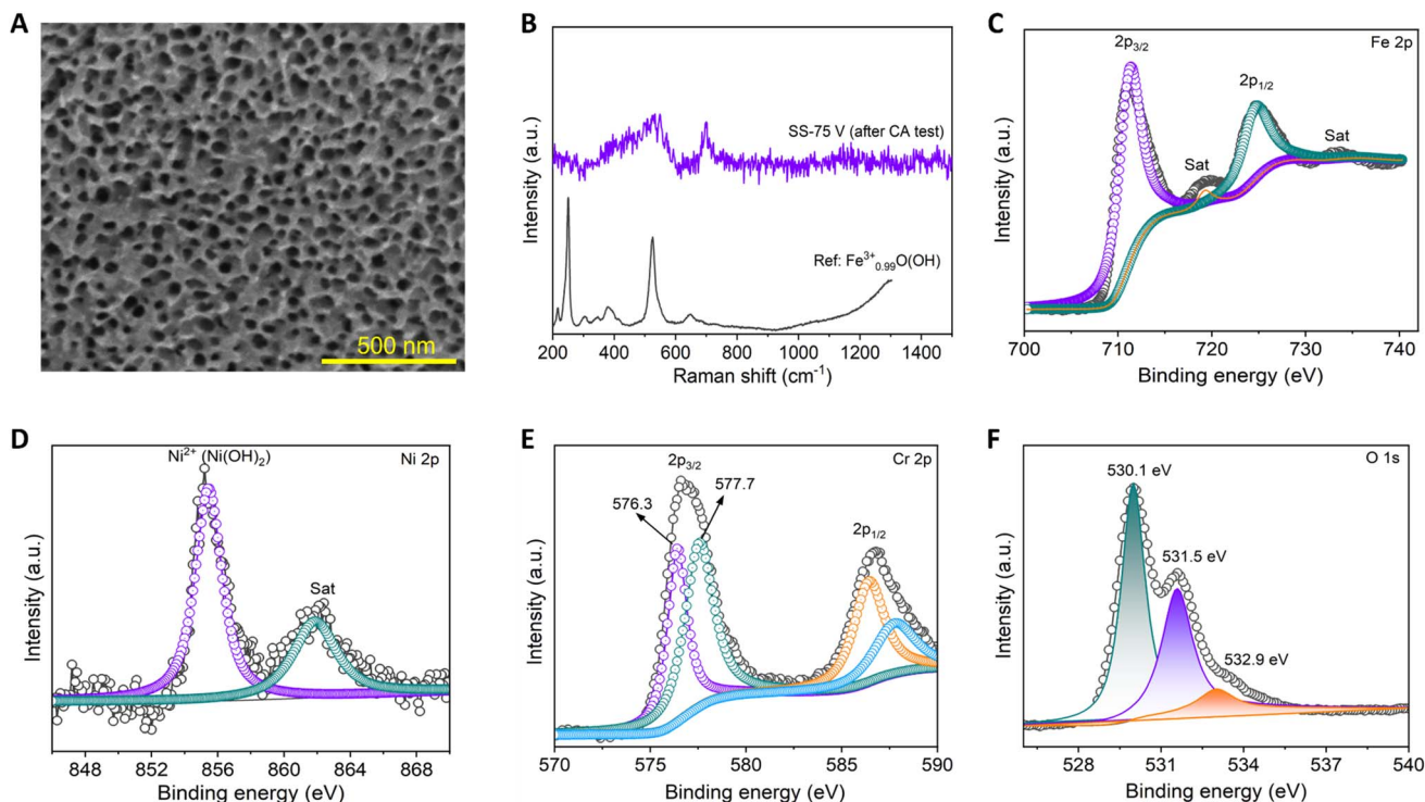
Fig. 4 Postcatalytic characterization of anodized SS-75 V electrode. (A) SEM image of after long-term stability test (magnification of 500 nm). (B) Raman spectra of SS-75 V electrode after CA testing. (C–F) Fe, Ni, Cr, and O valence state in SS-75 V electrode (after stability) examined by XPS analysis. (C) Fe 2p; (D) Ni 2p; (E) Cr 2p; (F) O 1s.
