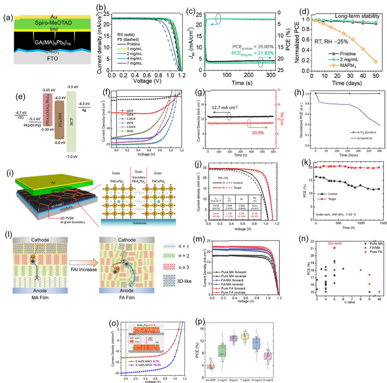
Fig. 4 (a) The quasi-2D ACI GA(MA) n Pb 5 I 3n+1 ( n = 5 ) based PSC device structure. (b) J - V curves of PSCs with and without (pristine) Iml treatment in both forward and reverse scans. (c) PSC's stabilized power output was measured at the MPP at a bias voltage of 0.948 V. The untreated (pristine) and treated samples contained 2 mg mL -1 Iml. (d) Stability of PSCs with and without (2 mg mL -1 ) Iml treatment and PSCs based on MAPbI 3 . (a)–(d) Reproduced with permission. 68 Copyright 2022, ACS. (e) PVSC device energy band alignment, (f) J - V curves of the devices with varying NH 4 SCN concentrations, (g) PSCs' photocurrent, (h) PSC devices' stability was tested in both an N 2 glove box and an environment with a humidity of 55% based on the (PEA) 2 (MA) 4 Pb 5 I 16 ( n = 5 ) perovskite film. (e)–(h) Reproduced with permission. 69 Copyright 2018, Wiley. (i) Device schematics that use a polycrystalline 3D perovskite film with 2D perovskites at the grain boundaries. (j) J - V curves. (k) Evolution of the PCE of the target and control. The devices were kept in a controlled-humidity environment that was dark. (i)–(k) Reproduced with permission. 148 Copyright 2018, Nature. (l) MA and FA-based schematics of 2D perovskites' crystal orientation and phase distribution in oblique and graded vertical alignments. (m) J - V curves for the best pure MA, FA/MA, and pure FA devices while scanning forward and backward. (n) High-efficiency, low-dimensional perovskite solar cell PCE is summarised. (l)–(n) Reproduced with permission. 70 Copyright 2022, Wiley. (o) J - V curves for 0 and 6 mol% MACl PSC champion devices. The inset schematic shows how MACl doping changes stacked perovskite films. Reproduced with permission. 149 Copyright 2020, ACS. (p) PCE statistics of PSCs that did not contain spiro-OMeTAD, broken down according to the different conditions of M2P precursor solution. Reproduced with permission. 150 Copyright 2020, Wiley.
