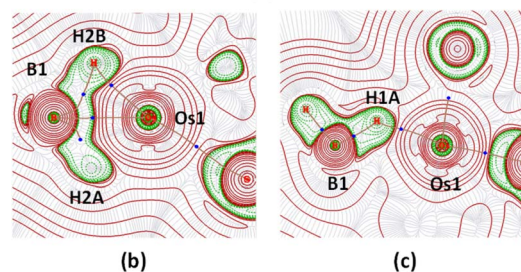
Fig. 8 (a) 3c–2e bonding interaction along the Os–H–B plane in 5' (isovalue 0.004 [e bohr -3 ] 1/2 ); (b and c) contour-line diagram of the Laplacian of the electron density along the Os–H–B planes in 5' and trans - 6 , respectively.
