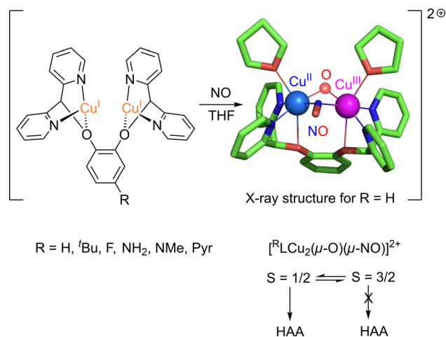
Fig. 10 Synthesis of [\text{R}'\text{LCu}_2(\mu\text{-O})(\mu\text{-NO})]^{2+} species and influence of the spin state on HAA reactivity from ref. 73 and 74.
