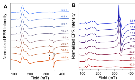
Fig. 3 CW EPR spectra ( \nu = 9.37 GHz, P_{\mu\text{W}} = 20 mW) of (A) \text{NiFd-CN} and (B) \text{NiFd-CO} at the indicated temperatures. Spectra were normalized to temperature using a standard Curie dependence [ I \propto T ]. * denotes small ( <5\% ) amount of contaminating S = 1/2 [\text{Fe}_4\text{S}_4]\text{-CN Fd} .
