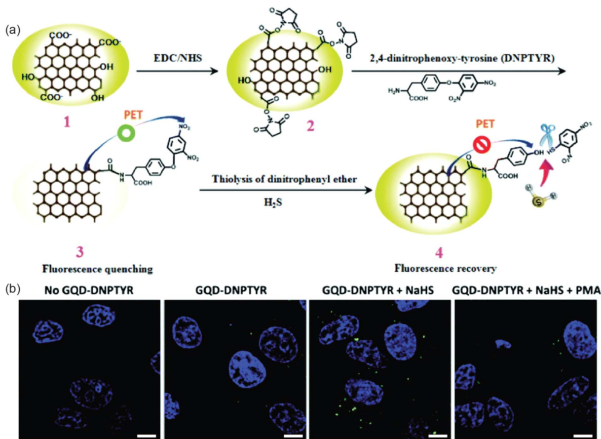
Fig. 10 (a) Schematic illustrations of the synthesis and photoluminescence quench mechanisms of GQD-DNPTYR. (b) Confocal images of MCF-7 cells treated with modified GQDs. Scale bar = 10 μm. Reproduced with permission reproduced with permission from ref. 207. Copyright © The Royal Society of Chemistry 2018.
