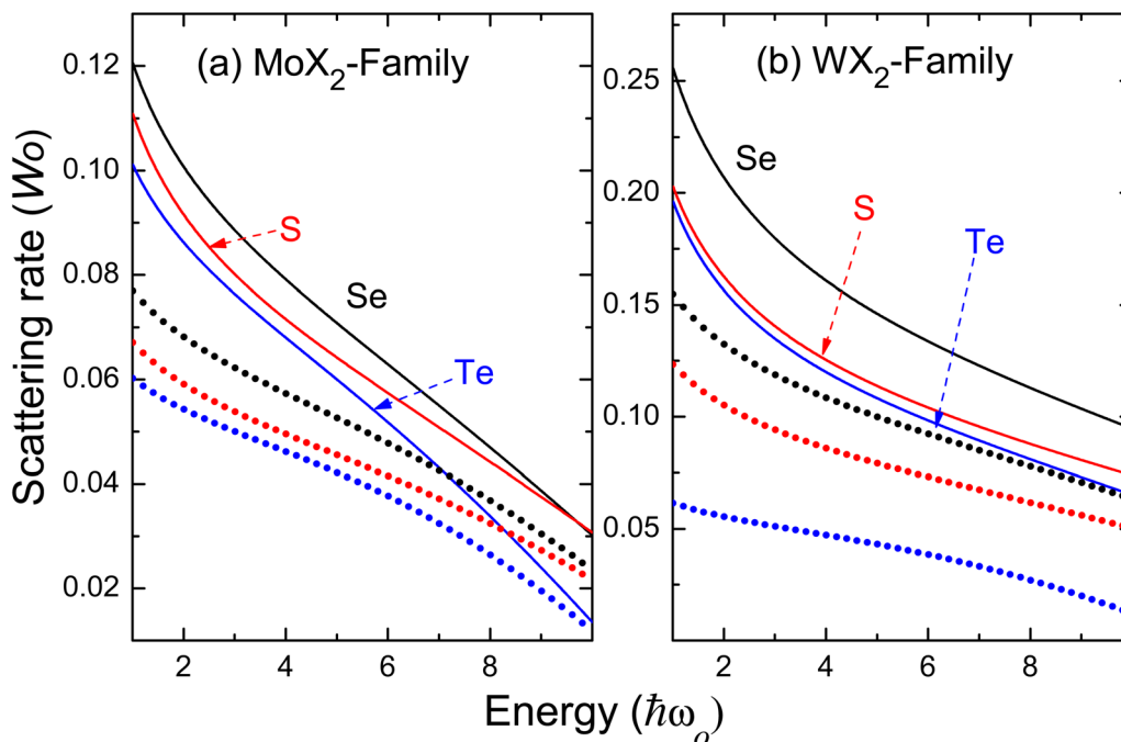
Fig. 9 Scattering rate as a function of the reduced energy E/\hbar\omega_0 for the (a) \text{MoX}_2 and (b) \text{WX}_2 families. Straight lines represent the ML samples ( \omega_0 = \omega_{E'} ), dots correspond to 2ML materials ( \omega_0 = \omega_{Eul} ). The parameters in Tables 1–3 are used, the results are given in units of W_0 (20) for the ML parameters.
