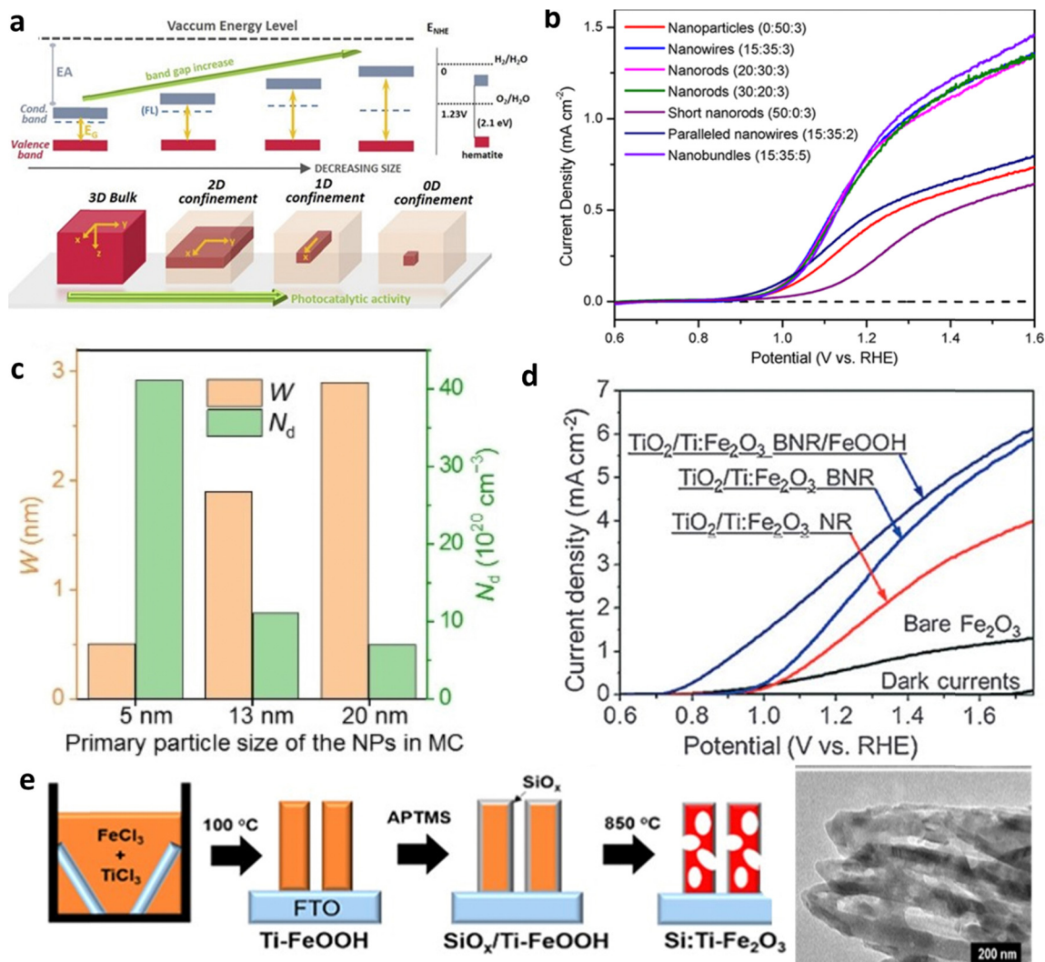
Fig. 8 Impact of nanostructuring and morphology. (a) Effect of particle size on bandgap and photocatalytic activity. Reproduced from ref. 79 with permission from APL Materials, copyright 2020. (b) J-V curve analysis of different nanostructured hematite photoanodes. Reproduced from ref. 83 with permission from John Wiley and Sons, copyright 2017. (c) Space charge region ( W ) and charge carrier density ( N_d ) profile of nanoparticles. Reproduced from ref. 82 with permission from John Wiley and Sons, copyright 2020. (d) J-V curve analysis of unbranched nanorod (NR) and branched nanorod (BNR) Ti-doped hematite photoanodes. (e) Fabrication of porous \text{Si:Ti-Fe}_2\text{O}_3 . Reprinted with permission from ref. 83, Copyright 2022 American Chemical Society.
