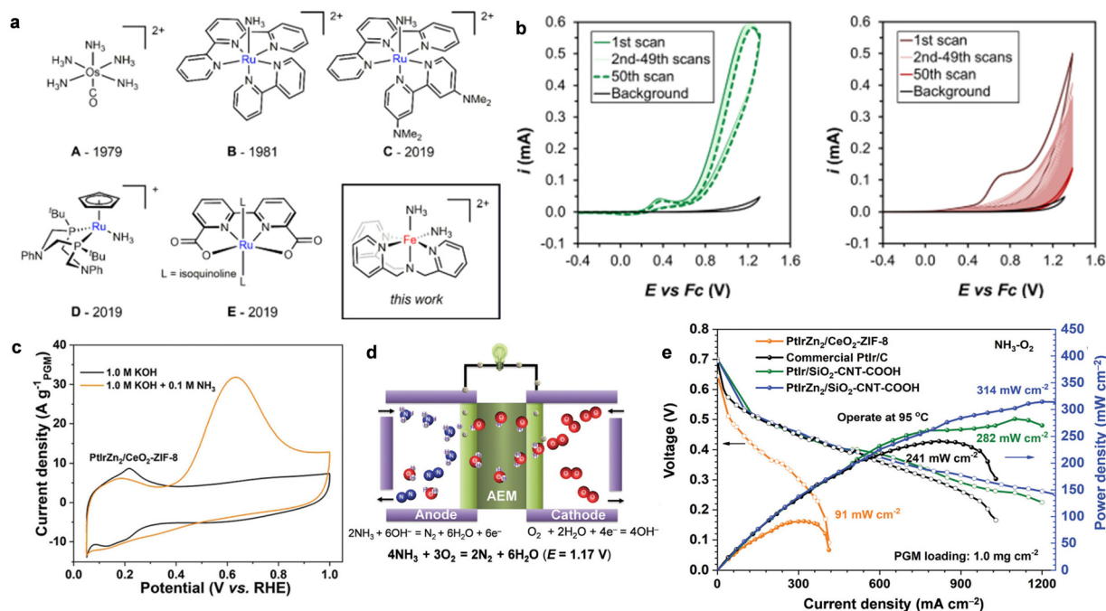
Fig. 6 (a) Representative molecular complexes that catalyze the AOR. (b) The cycling of 2.5 mM [\text{TPA}]\text{Fe}(\text{MeCN})_2\text{OTf}_2 (left) or 2.5 mM \text{FeOTf}_2 (right) in \text{CH}_3\text{CN} + 50 mM \text{NH}_3 or \text{CH}_3\text{CN} + 50 mM \text{NH}_4\text{OTf} solution. Reproduced with permission from ref. 84 Copyright 2019, ACS publications. (c) CV curves of the AOR activity of PtIrZn 2 /CeO 2 -ZIF-8 in the presence and absence of \text{NH}_3 . (d) A schematic view of the DAFC single cell. (e) The polarization curves and power density curves of DAFCs with different anode catalysts. Reproduced with permission from ref. 38 Copyright 2020, The Royal Society of Chemistry.
