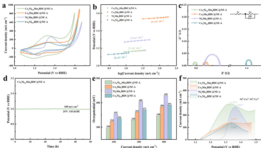
Fig. 5 Electrocatalytic OER in 1 M KOH. (a) The cyclic voltammograms of different catalysts. (b) Tafel plots obtained from (a). (c) EIS Nyquist plots. (d) Long-term stability curve for achieving 100 mA cm -2 with Co 1 Ni 0.5 Mn 1 BDC@NF-A. (e) Overpotentials needed at current densities of 100, 300 and 500 mA cm -2 for different samples. (f) Comparison of oxidation peaks on partial CV curves.
