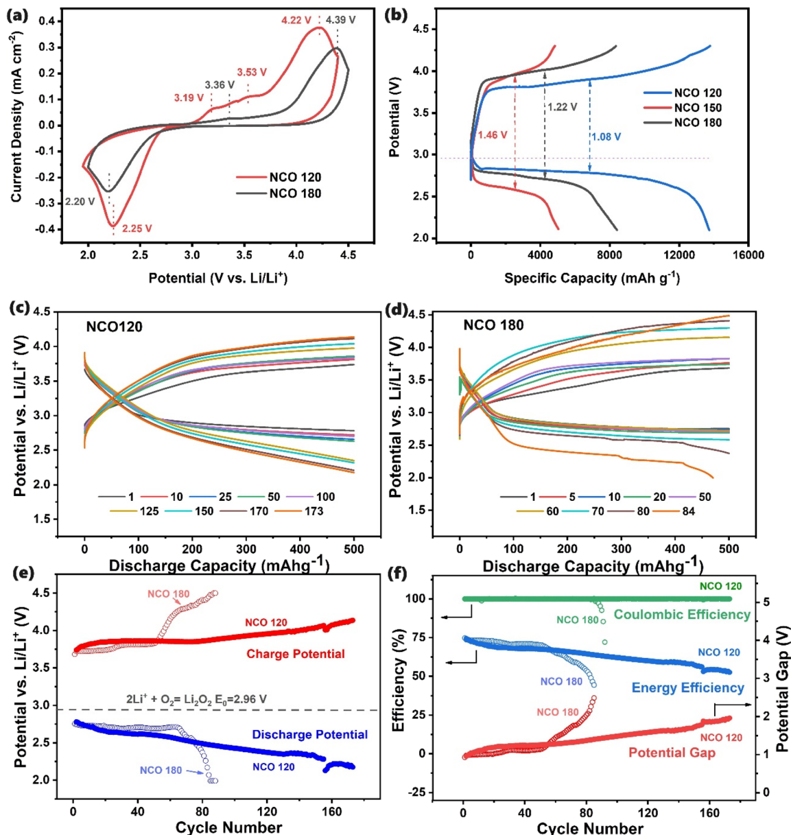
Fig. 4 (a) CV analysis @0.2 \text{mV s}^{-1} and (b) full discharge–charge @100 \text{mA g}^{-1} , and selected discharge–charge curves of (c) NCO 120 and (d) NCO 180 cathode-based LABs operated at 100 \text{mA g}^{-1} for a limited capacity of 500 \text{mA h g}^{-1} . (e and f) Cycle life and performance analysis of LABs with NCO 120 and NCO 180 based cathodes with cut-off discharge capacity of 500 \text{mA h g}^{-1} with 1 M LiTFSI dissolved in TEGDME electrolyte.
