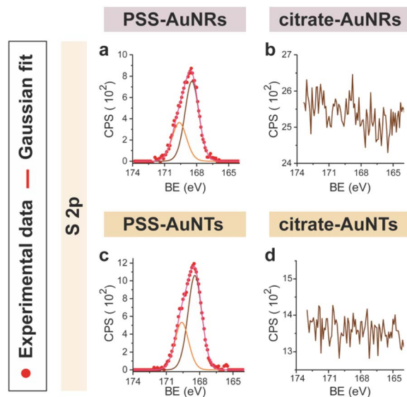
Fig. 4 XPS high-resolution spectra in the S 2p region for: (a) PSS-AuNRs, (b) citrate-AuNRs, (c) PSS-AuNTs, (d) citrate-AuNTs.
