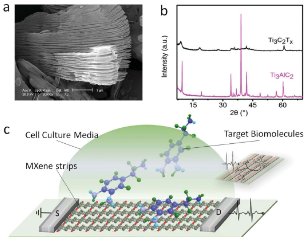
Fig. 17 Characterization of bulk MXenes. (a) SEM image of the multilayer structured MXene. (b) XRD patterns of the transition from Ti_3AlC_2 to Ti_3C_2T_x . (c) Schematic of a biosensing device based on MXene field effect transistors (copyright 2016 John Wiley and Sons). 151
