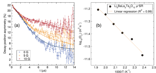
Fig. 6 (a) μ + SR raw data collected at room temperature at zero field (blue) and applied fields of 5 G (yellow) and 10 G (red) and fit the data using the Keren function (solid line) for the undoped Li 6 BaLa 2 Ta 2 O 12 garnet material. (b) Arrhenius plot of the diffusion coefficient calculated from μ + SR for the undoped Li 6 BaLa 2 Ta 2 O 12 garnet. The calculated activation energy from it is 0.16(1) eV.
