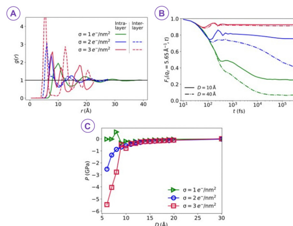
Fig. 3 (A) The xy pair correlation g(r) between ions indicates that as the surface charge densities \sigma increase at fixed separation D = 8 Å, ions become closer together and their positions become more correlated. (B) Intermediate scattering functions F_s(q_z, t) for the ions measured for the same \sigma values as in (A) and for two different surface separations D = 10 and 40 Å. Here, the stronger spatial correlations with increasing surface charge density in (A) correspond to increasingly correlated dynamics and more strongly localized ions. (C) The increasing correlations drive the overall pressure between the confining walls to become increasingly attractive, reaching P_{\min} \approx -6 GPa at \sigma = 3 e^- \text{ nm}^{-2} (reproduced from ref. 11 with permission from AAAS, copyright 2021).
