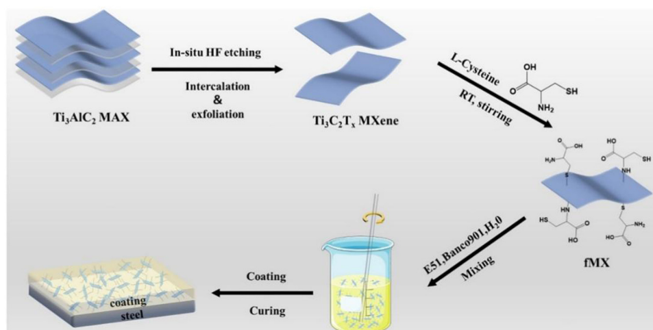
Fig. 9 The preparation process of MXene (Ti 3 C 2 T x ), fMX and the composite coating. Reproduced with permission from ref. 143. Copyright 2021 Elsevier.
