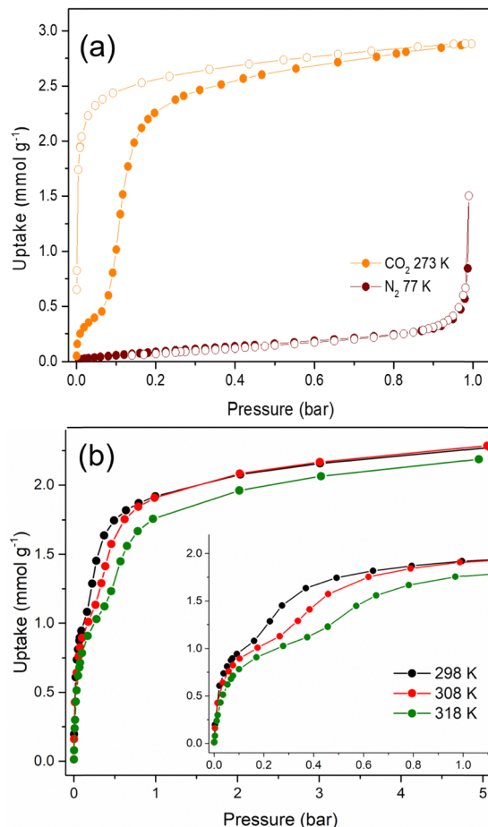
Fig. 2 Low pressure \text{N}_2 (77 K, wine) and \text{CO}_2 (273 K, orange) adsorption/desorption isotherms (a) and high pressure \text{CO}_2 adsorption isotherms collected at 298 K (black), 308 K (red) and 318 K (green) (b). The isotherms were collected using 60 s of equilibration time.
