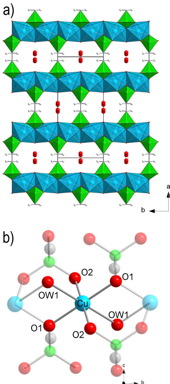
Fig. 1 Polyhedral representation of the crystal structure of as synthesized Cu-EtP, viewed along the c axis (a) and detail of the local connectivity around the \text{Cu}^{\text{II}} atoms (b, atoms not directly connected to the central Cu are shaded to highlight the coordination sphere of the central atom). Colour code: Cu, cyan; P, green; C, grey; O, red; H, white.
