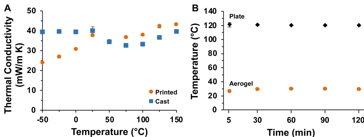
Fig. 8 (A) Thermal conductivity of cast and printed aerogels at various temperatures. (B) Temperature of plate and aerogel over time. Error bars indicate standard deviation ( n = 3 ).
