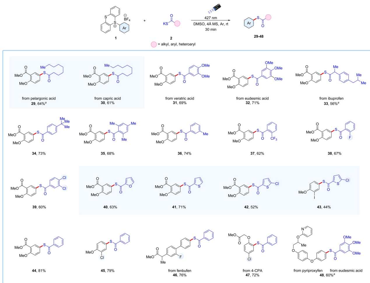
Scheme 2 Reaction conditions: aryl thianthrenium salt 1 (0.3 mmol), potassium thioacetate salt 2 (2 equiv., 0.6 mmol), 4 Å MS (60 mg), in 1.5 mL DMSO, were irradiated with 427 nm Kessil Lamp (40 W) at room temperature under argon for 30 min. a 2 h.
