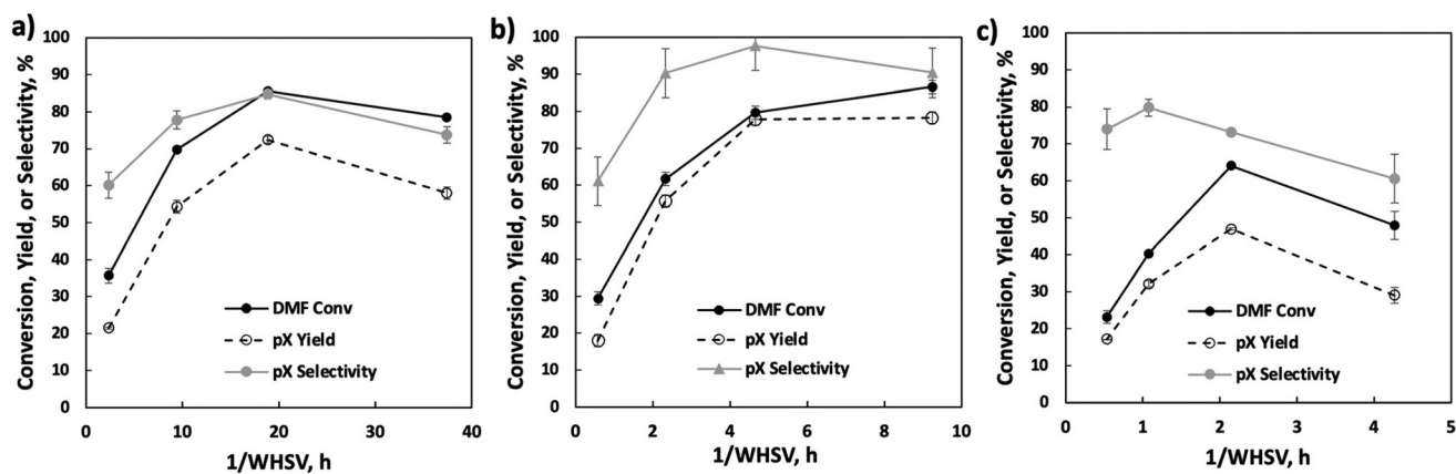
Fig. 4 Reactor performance at various 1/WHSV using 5 wt% (2.36 h, 9.43 h, 18.86 h, and 37.4 h, panel a), 20 wt% (0.57 h, 2.33 h, 4.66 h, and 9.24 h, panel b), and 40 wt% (0.54 h, 1.07 h, 2.15 h, and 4.26 h, panel c) DMF in n -heptane liquid feed. Conditions: 375 °C, 750 psig back pressure, 0.5 g P-BEA(25).
