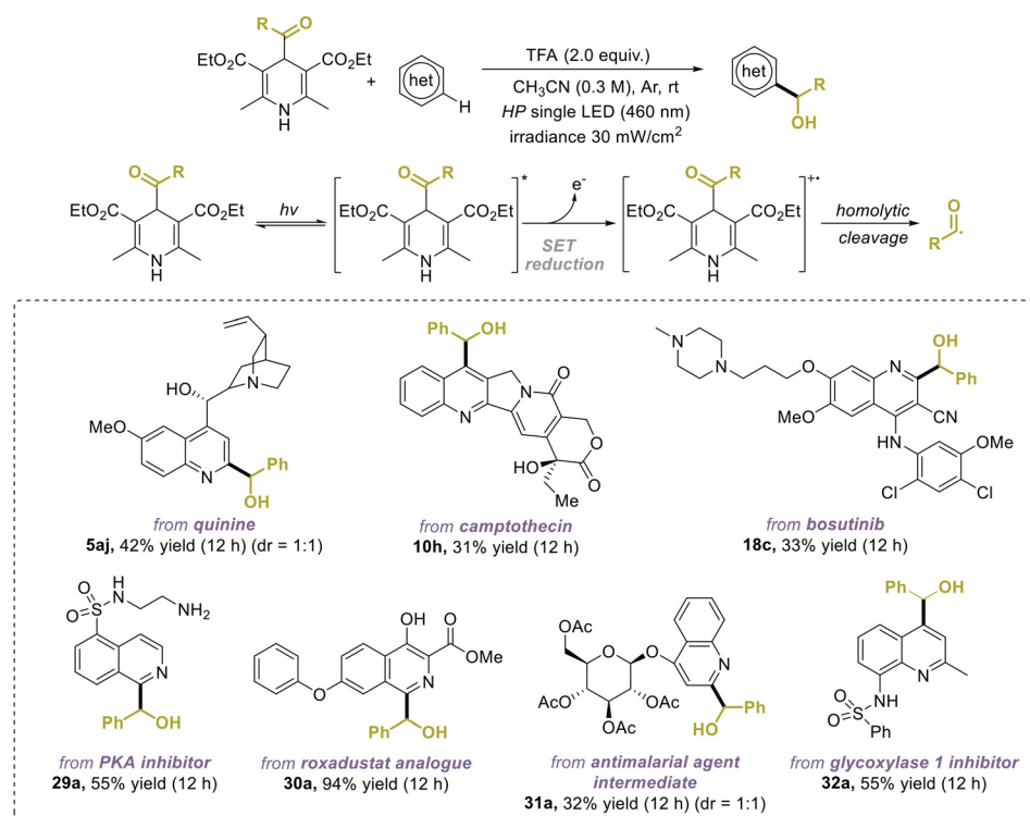
Fig. 38 Photo-mediated Minisci α-hydroxyalkylation with acyl-DHPs.
