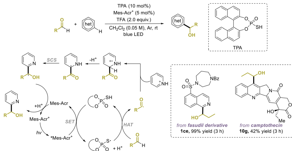
Fig. 37 Photocatalytic Minisci α-hydroxyalkylation with aldehydes.
