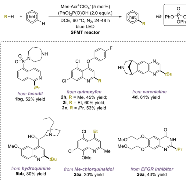
Fig. 27 Photocatalyzed Minisci alkylations with alkanes assisted by SFMT reactors.
