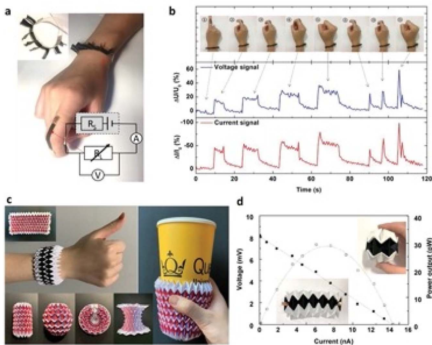
Fig. 16 (a) A self-powered thermoelectric (TE) device in the form of a “bracelet”. The device incorporates 8 TE couples and is designed to generate power to operate a strain-sensing component that functions as a motion detector for the index finger. (b) It demonstrates responsiveness to different finger positions by utilizing a temperature difference of about 20 °C. (c) The concept of TE devices with multiple couples is introduced, taking inspiration from the origami “magic ball” design. (d) Power output of a 6-couple TE device when subjected to a 20 °C temperature difference. Reproduced from ref. 78 with permission of Wiley.
