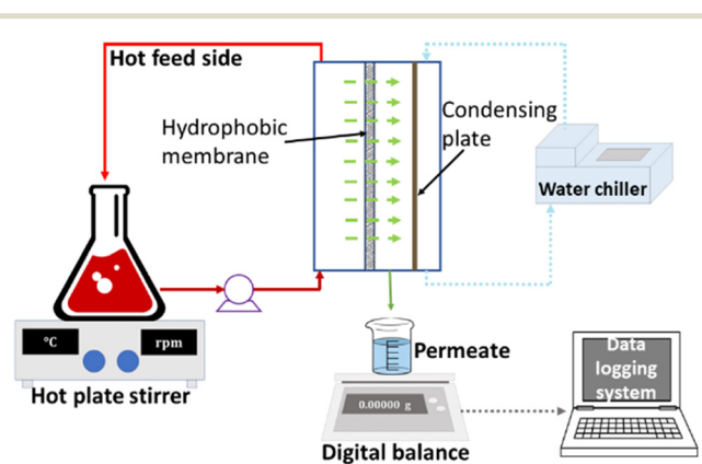
Fig. 1 Schematic diagram of the experimental rig of the AGMD process.
