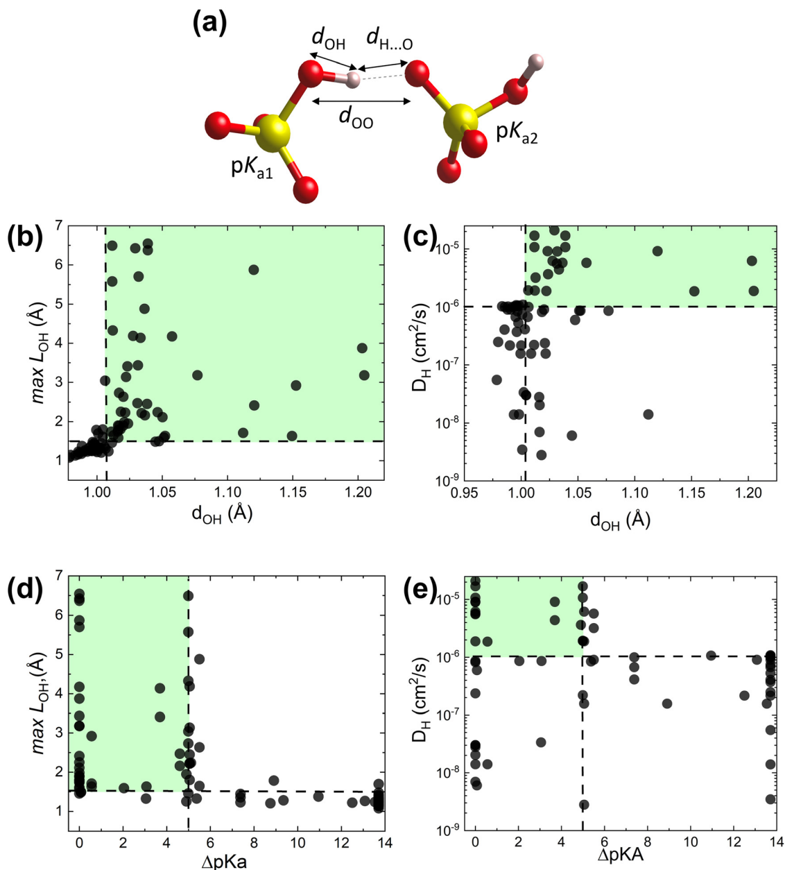
Fig. 2 AIMD results from the initial dataset to extract proton transfer descriptors. (a) Schematic showing d_{\text{OH}} , d_{\text{H}\dots\text{O}} , d_{\text{OO}} and \text{pK}_a for donor and acceptor groups in a solid acid (color code: S is yellow, O is red, and H is pink). (b) Maximal distance travelled by the proton from its initial donor atom during the AIMD run, L_{\text{OH,max}} , vs. the maximal initial O–H bond length, d_{\text{OH}} . (c) Proton diffusivity, D_{\text{H}} , vs. d_{\text{OH}} . (d) L_{\text{OH,max}} vs. \Delta\text{pK}_a . (e) D_{\text{H}} vs. \Delta\text{pK}_a . All data at 700 K (the trajectory length is 25 ps). Dashed lines correspond to the selected cut-offs: D_{\text{H}} cut-off is set to 10^{-6} \text{ cm}^2 \text{ s}^{-1} , which corresponds to about 0.02 \text{ S cm}^{-1} conductivity at 700 K and is above the AIMD accuracy limits (for further details see Computational methods, Section S1 in the ESI†).
