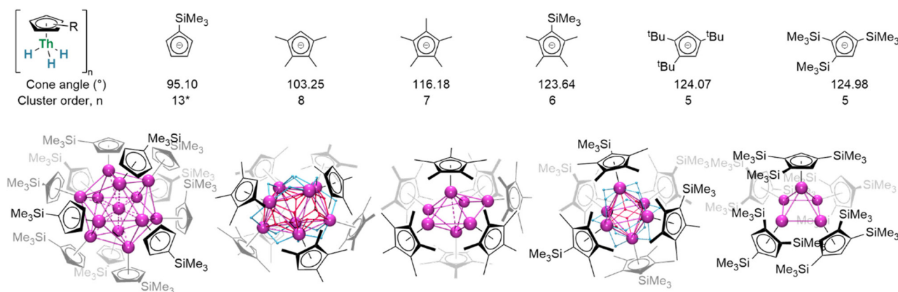
Fig. 20 Cluster order decreases with increasing with cyclopentadienyl ligand cone angle, measured from solid state structures. * The Cp' ligand results in a complex cluster of the form ((\text{Cp}'\text{Th})_3(\text{H})_{10})_4\text{Th} in which the position of the hydrides is unknown. Despite its non-standard nature it is clear that this ligand can, and does, facilitate for formation of higher-order clusters than its smaller analogues. This cluster is also reminiscent of the structure of binary hydride \text{Th}_4\text{H}_{15} .
