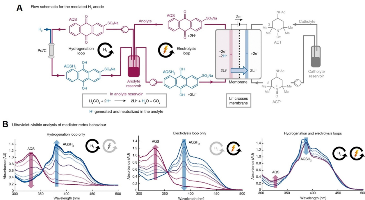
Fig. 18 (A) Schematic of mediated H 2 anode by pairing the thermal hydrogenation of AQS and the electrochemical oxidation of AQS(H 2 ) in real time. (B) In situ UV-Vis spectra of the redox speciation of AQS and AQS(H 2 ) species in the anolyte reservoir for various processes, such as hydrogenation-only or electrolysis-only loop, or both loops operating simultaneously. Reproduced with permission from ref. 215. Copyright 2023 Springer Nature.
