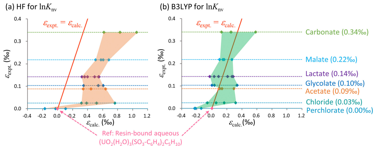
Fig. 3 Calculated \varepsilon values based on \ln K_{\text{nv}} obtained using the (a) HF and (b) B3LYP methods along with experimental data for the U(vi)–U(vi) system. The horizontal axis shows the calculated values relative to \text{UO}_2(\text{H}_2\text{O})_3(\text{SO}_3\text{-C}_6\text{H}_4)_2\text{C}_5\text{H}_{10} while the vertical axis shows the experimental values relative to the aqueous \text{UO}_2^{2+} complex bound to the cation exchange resin. The red solid line indicates the scenario in which the calculated and experimental values are equal. The areas bounded by the values calculated using the HF and B3LYP methods are shaded orange and green, respectively. The dotted lines parallel to the horizontal axis represent the experimental values for each species as described on the right while the quantities in parentheses indicate the experimental data. The numerical data are also summarized in Table 3.
