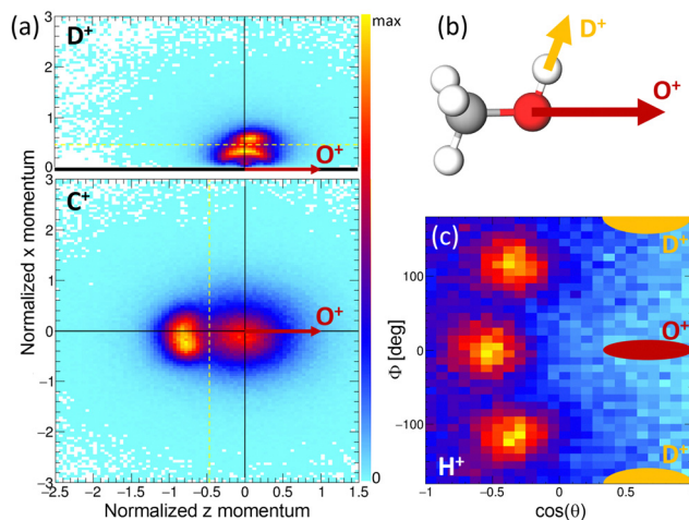
Fig. 7 Left row: experimental ion momenta in the molecular frame defined by the emission direction of the O^+ ion (defining the z axis) and the D^+ ion (spanning together with the O^+ the xz plane and defining the positive x direction), measured at SQS/EuXFEL. In the top panel, the momentum of the D^+ ion is depicted in that frame, in the bottom panel the momentum of the C^+ ion is shown. Right row: sketch of the breakup of the methanol-OD molecule (top panel). The bottom panel on the right shows the three-dimensional angular emission distribution of the measured protons in the coordinate frame spanned by the O^+ and D^+ ions [yellow lines in panels (a) and (b) indicate filters for the ion momenta used in panel (c), see the text for details].
