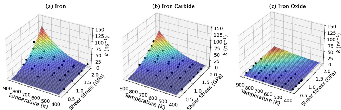
Fig. 13 3D fits of TCP decomposition rate as a function of temperature and shear stress for (a) \alpha -Fe(110), (b) \text{Fe}_3\text{C}(010) and (c) \text{Fe}_3\text{O}_4(100) surfaces.
