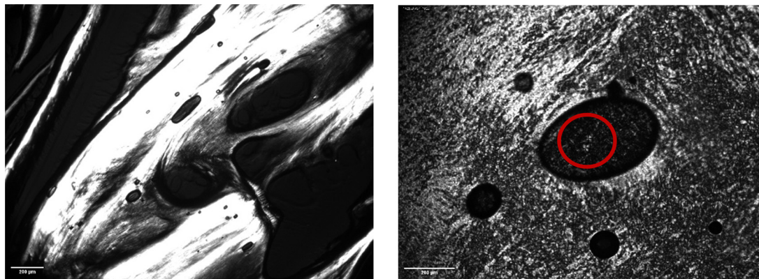
Fig. 5 Polarised-light microscope images of CAOC at 15 °C, showing birefringence and a Maltse cross pattern (red circle) indicative of a lamellar liquid crystalline phase. The images are taken at different points of the same sample slide with 4× magnification (left) and 10× magnification (right).
