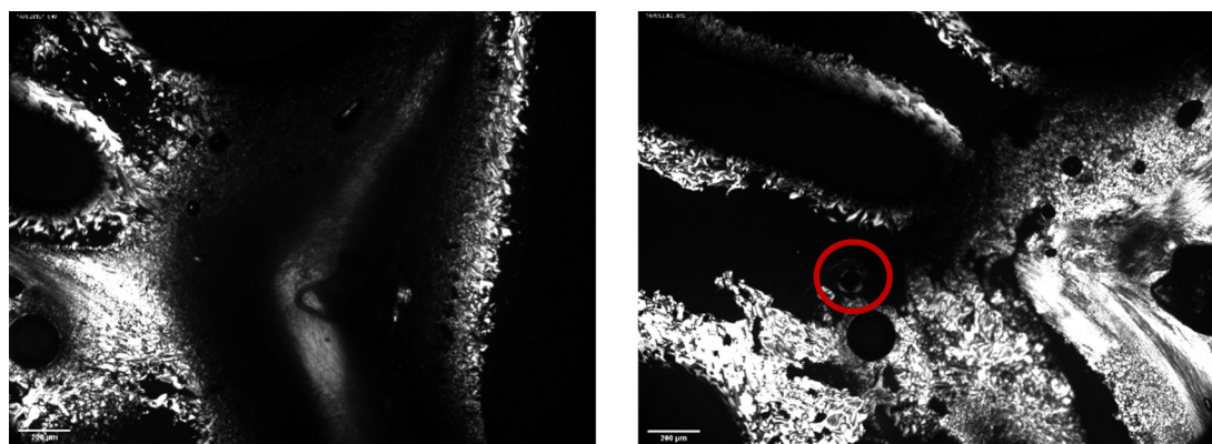
Fig. 6 Polarised-light microscope images of BTMAAOC at 5–10 °C, showing birefringence and a Maltse cross pattern (red circle) indicative of a lamellar liquid-crystalline phase. The images are taken at different points of the same sample slide with 4× magnification.
