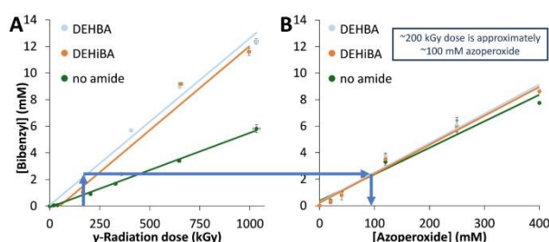
Fig. 5 A) Absorbed gamma-radiolysis dose compared to B) radical assay azoperoxide concentration showing estimated correspondence using bibenzyl formation in toluene. Error bars represent results of trials performed in triplicate.
